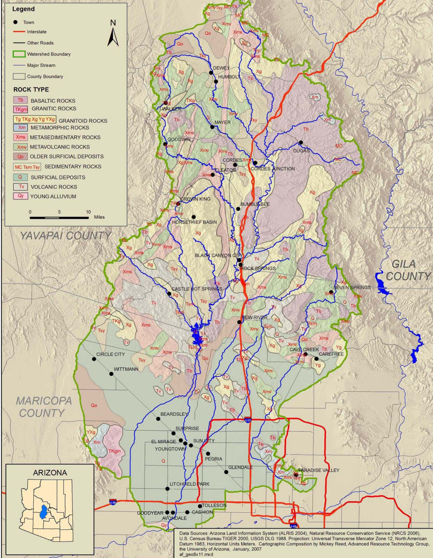
Fig. 2-1: Agua Fria River Watershed Geology
